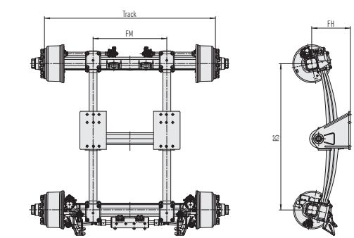
Boogie suspension unit
